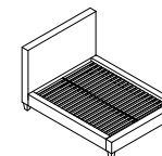
Q2, QR, QW 54" Complete Queen Bed w/ Rails, Footboard, Wood Slats 67 x 92 x 54" 170 x 234 x 137 cm
